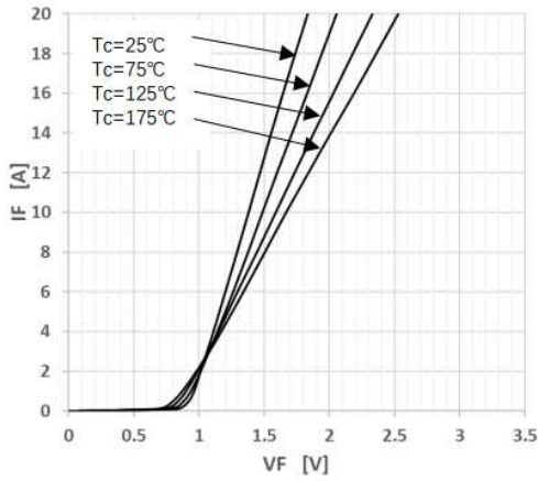
Figure 1 Forward Characteristics
