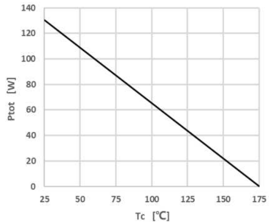
Figure 4 Power Dissipation
